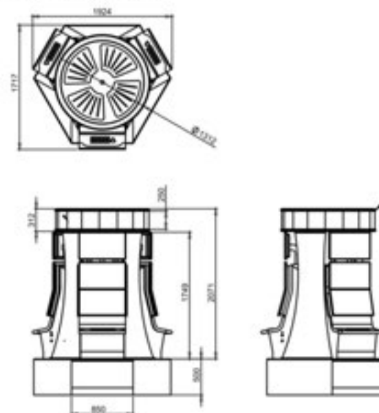
Sign / bank dimensional details
